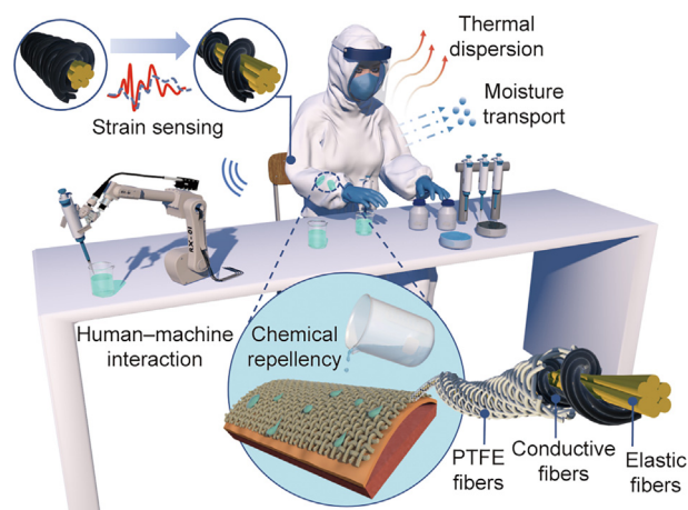
Fig. 1. Schematic and working mechanism of stretchable hierarchical core-shell yarns (HCSYs)/hierarchical core-shell structured yarn-based textiles (HCSTs). Schematic of the HCSYs/HCSTs with the hierarchical core-shell structure used to integrate the functional application of chemical resistance, real-time motion detection, human-machine interaction, and tunable thermal management in high-risk environments. PTFE: polytetrafluoroethylene.
