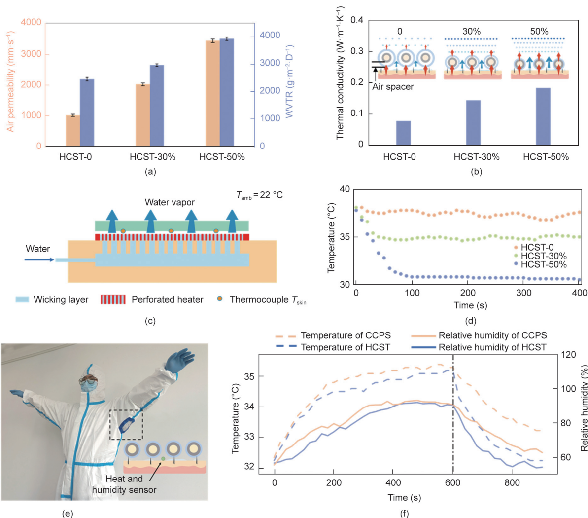
Fig. 6. Tunable thermoregulation function of HCST. (a) Air permeability and moisture permeability of HCSTs at different strain ratios (0, 30%, and 50%, respectively). WVTR: water vapor transmission rate. (b) Thermal conductivity of HCSTs at different strain ratios (0, 30%, and 50%, respectively) at 25 °C. The inserted photographs show the working mechanisms of our HCSTs interacting with adjustable thermal conductive interfaces and separating domains with different mechanical actuation. (c) Schematic of the tunable thermal management test. T_{amb} : ambient temperature, T_{skin} : skin temperature. (d) Lower part temperatures of HCSTs at different strain ratios were measured by the thermocouple in a purpose-designed experimental environment. (e) Photograph of a person wearing a chemical protective suit with an integrated piece of HCST. (f) Comparison of the as-measured temperature and relative humidity of a person wearing a CCPS with and without HCST integration during exercising and releasing states.
