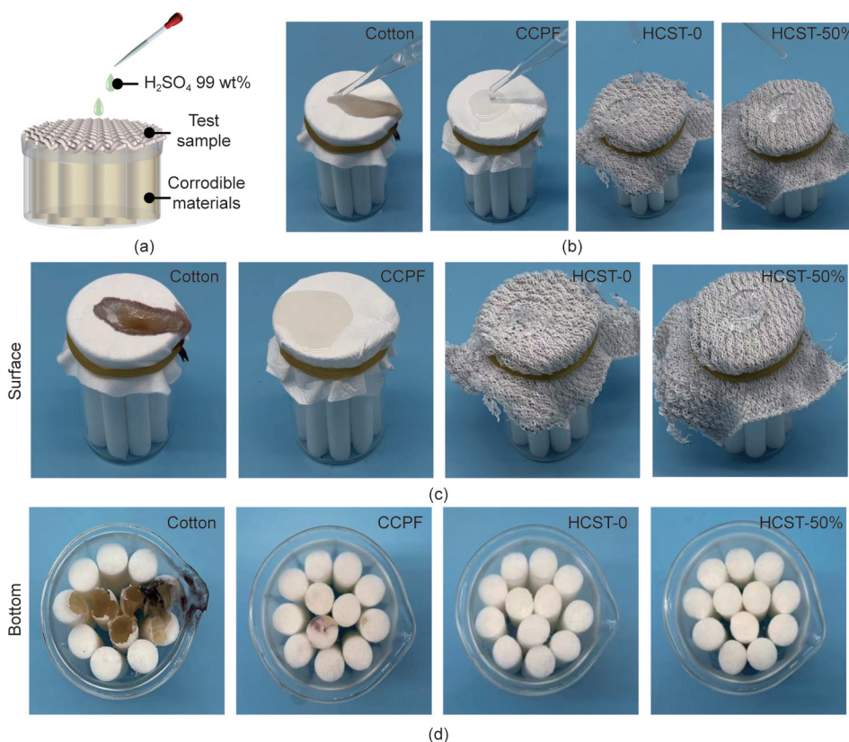
Fig. 3. Chemical resistance characterization of HCST. (a) Schematic of self-built chemical resistance test device. (b) Optical images of the sample surface after dipping by 1 mL of 99 wt% H 2 SO 4 . (c) Optical images of the sample surface after being exposed to 99 wt% H 2 SO 4 for 10 min. (d) Optical images of the corrodible materials after removing the covered fabrics.
