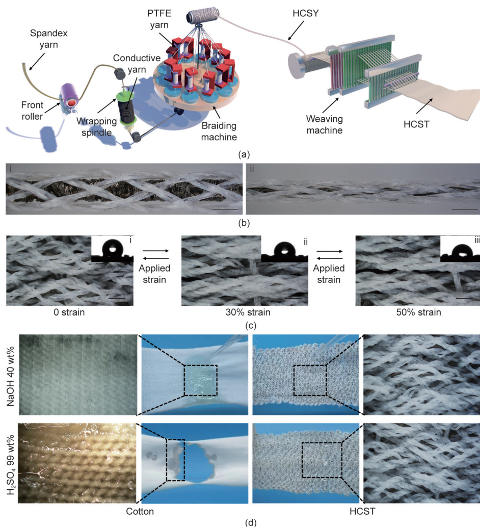
Fig. 2. Fabrication and characterization of HCSYs and HCSTs. (a) Schematic fabrication process of HCSYs and HCSTs. (b) Photograph of as-fabricated HCSYs (i) before and (ii) after stretching; scale bars: 1000 \mu\text{m} . (c) Optical images of an HCSTs piece subjected to the applied strains of (i) 0, (ii) 30%, and (iii) 50%. The inserted photographs show the contact angles of a 40 wt% NaOH droplet on HCST; scale bars: 500 \mu\text{m} . (d) Optical photographs showing the chemical resistance of HCSTs (contacted with 40 wt% NaOH; 99 wt% \text{H}_2\text{SO}_4 ); the scale bars in optical images and micrographs are 2 cm and 500 \mu\text{m} , respectively.
