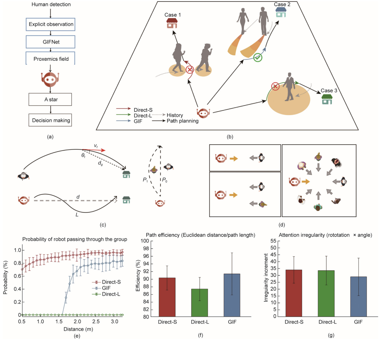
Fig. 6. The GIF for crowd-aware robot navigation. (a) Illustration of the pipeline of GIF-based navigation. Our method uses the GIF to guide robot path planning. (b) Illustration of three different path-planning methods in our experiments. The Direct-S and Direct-L methods are widely used robot navigation approaches that treat pedestrians as simple circular obstacles [60]. The Direct-S method treats pedestrians as small circular obstacles and often causes robots to disturb pedestrians. The Direct-L method treats pedestrians as large circular obstacles, resulting in sacrifices in navigation efficiency and a longer path. The GIF method treats the range of the predicted proxemics field as an obstacle. To ensure a fair comparison, we adopt the classic A-star path-planning method to evaluate the performance of the three methods. (c) Three metrics are used for evaluation. The robot path efficiency is the ratio between the robot's Euclidean distance d to the goal and the actual traveled distance L , which measures the robot navigation efficiency. The attention irregularity is the sum of the pedestrians' unnecessary rotation angle caused by the robot, which measures the robot's disturbance to pedestrians. The probability of the robot passing through the group P_0 is used to measure the disturbance the robot causes to the pedestrian group. (d) Illustration of the layout of our experiments. We evaluate three methods under three different scenarios: one robot with one person, one robot with two persons, and one robot with multiple persons. (e) The probability of the robot passing through a two-person group versus the inner distance between the two people in the two-person group. Our group-aware method can accurately identify groups (whose inner distance is usually less than 1.5 m) and prevent robots from passing through them. (f, g) A comparison of the (f) path efficiency and (g) attention irregularity. Our GIF-based method has the highest path efficiency and the lowest attention irregularity, which suggests that our method effectively prevents robots from disturbing pedestrians while maintaining the robot's driving efficiency. The error bars represent the standard deviation. \theta_i : the inner angle of the direction of the destination; d_g : and the direction of the current speed v_i .
