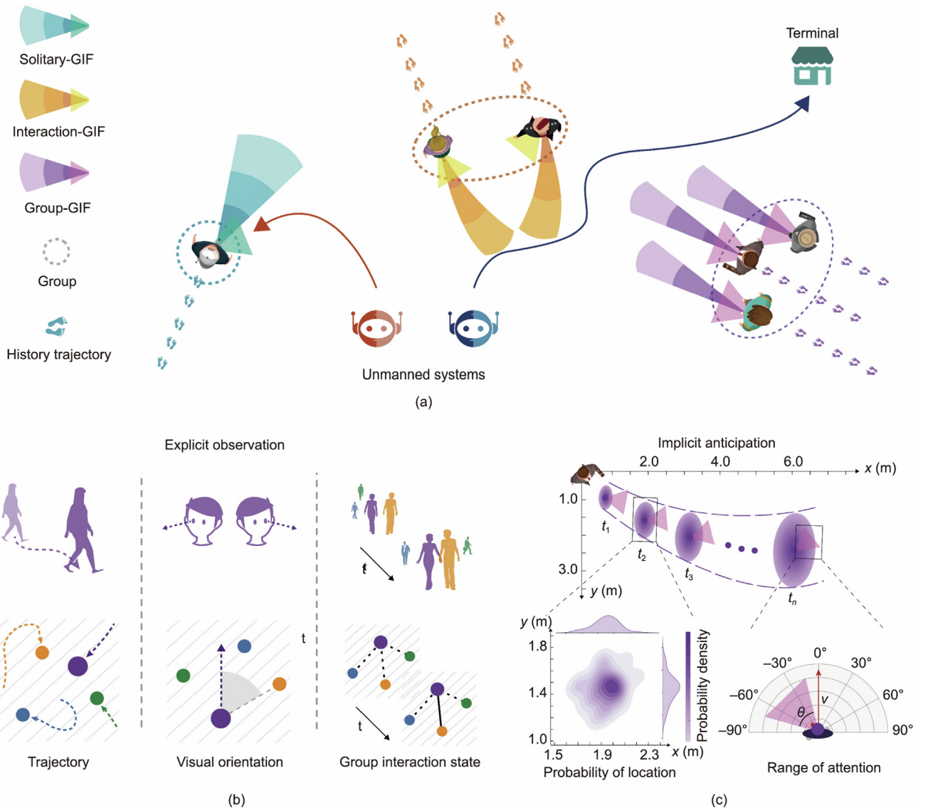
Fig. 1. The group interaction field (GIF). (a) The GIF represents implicit pedestrian anticipation; it consists of a proxemics field and an attention field, estimated from explicit observations. (b) Explicit observations consist of trajectory, visual orientation, and observable group interaction state. (c) The proxemics field and the attention field are represented by a sequence of two-dimensional (2D) probabilistic distribution maps and a sequence of angular ranges, respectively. Two representative applications are demonstrated in part (a); the GIF can help unmanned systems to either avoid disturbing pedestrians or attract pedestrians' attention. t_1, t_2, \dots, t_n : timestamp from the prediction sequence; n : n th timestamp; v : walking velocity; \theta : angular range of the attention field.
